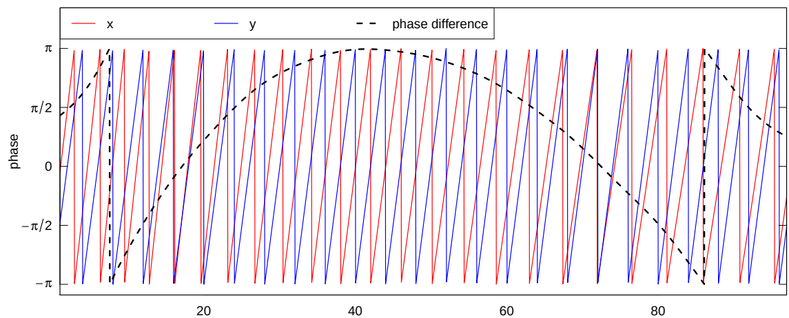
Figure 32: Phases and phase differences: asymmetry due to increasing period
