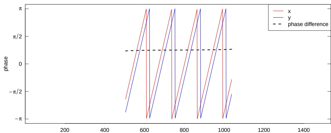
Figure 28: Phases and phase differences at period 128
