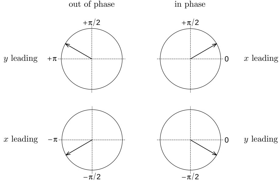
Figure 2: Phase-differences and their interpretation
