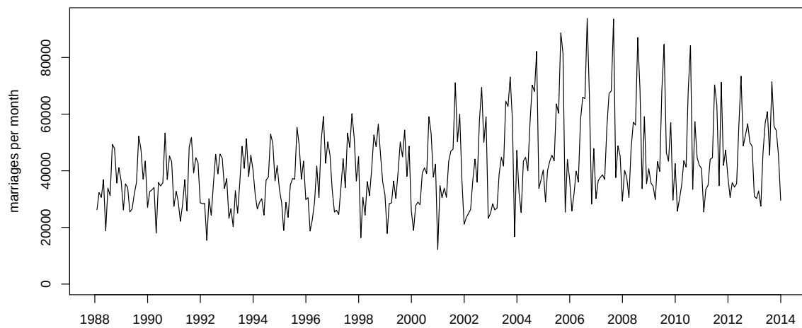
Figure 42: The series of monthly marriages (“Sunday-adjusted”)
