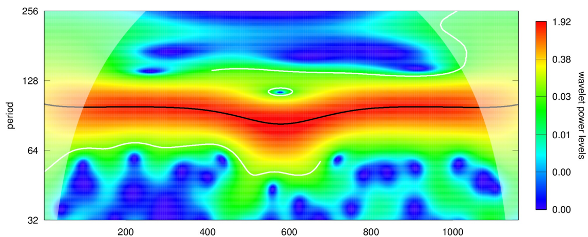
Figure 19: Power spectrum, plot gone wrong
