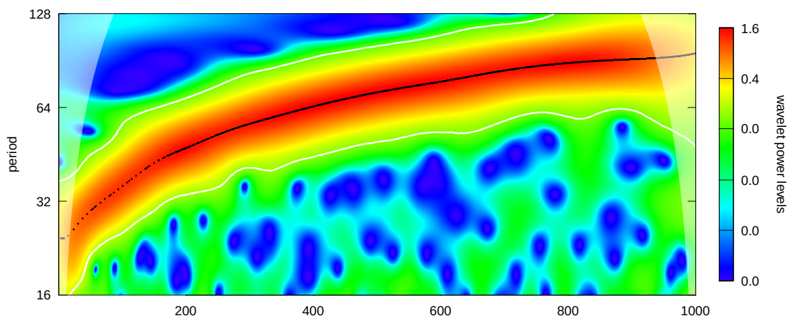
Figure 7: Wavelet power spectrum of the series with nonconstant period
