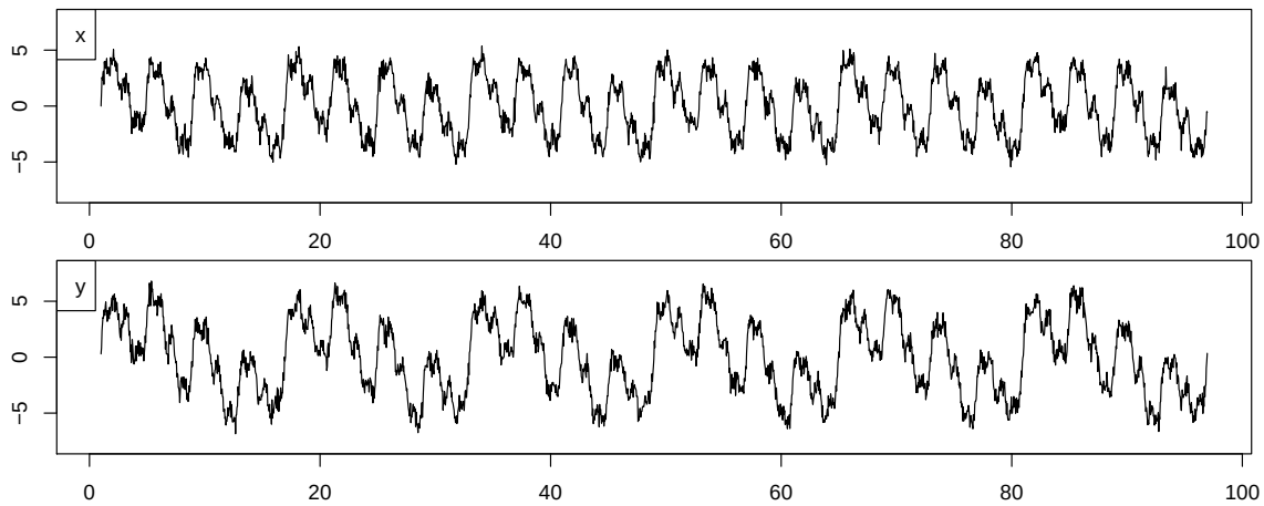
Figure 21: Two series with periods 1, 2, 4, 8, 16 and different amplitudes
