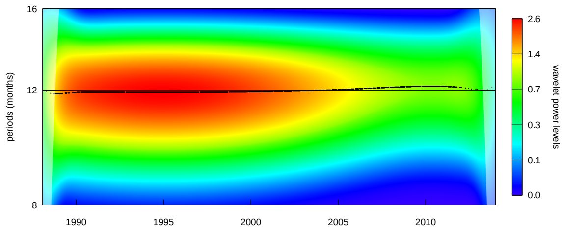
Figure 47: Power spectrum of simulated series
