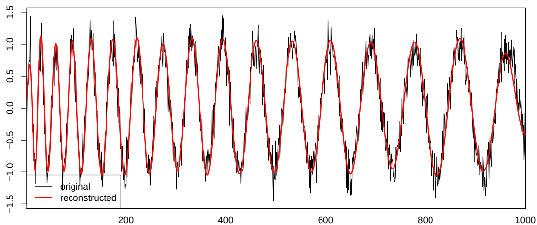
Figure 8: Reconstruction of the series with nonconstant period
