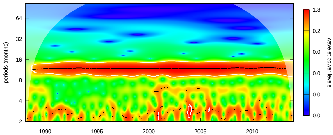
Figure 43: Marriages, the wavelet power spectrum
