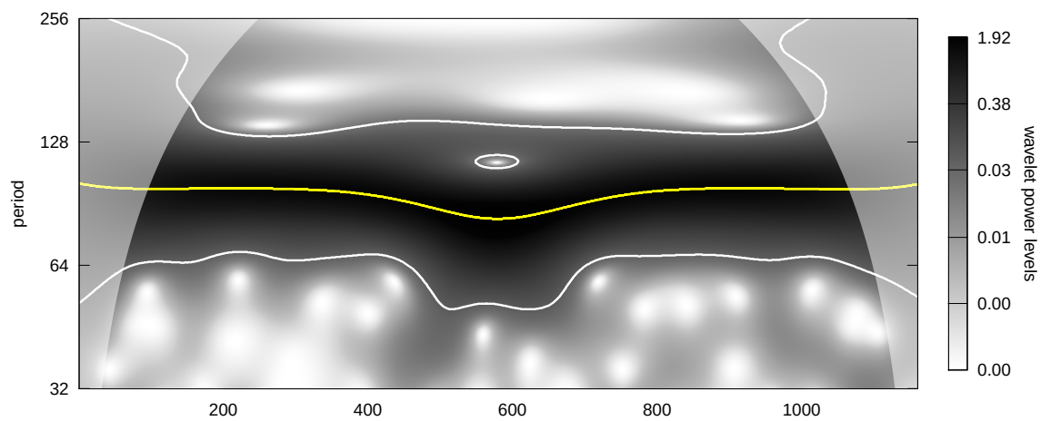
Figure 20: Power spectrum, grayscale, yellow ridge
