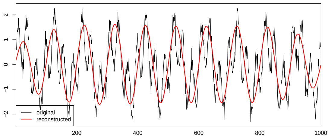
Figure 11: Reconstruction of the series with superposed periods, using only period 100
