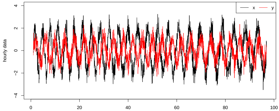
Figure 30: Two series, overlapping periods
