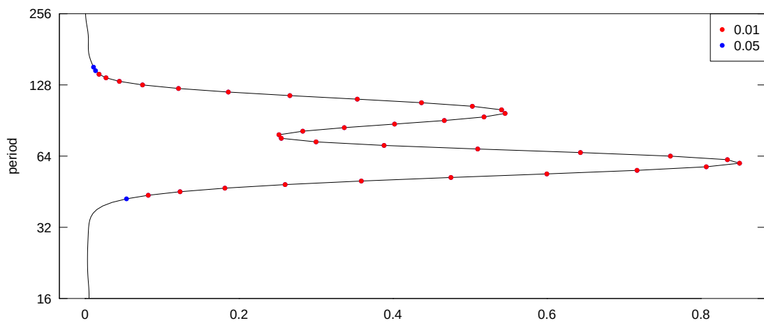
Figure 13: Average power, series x
