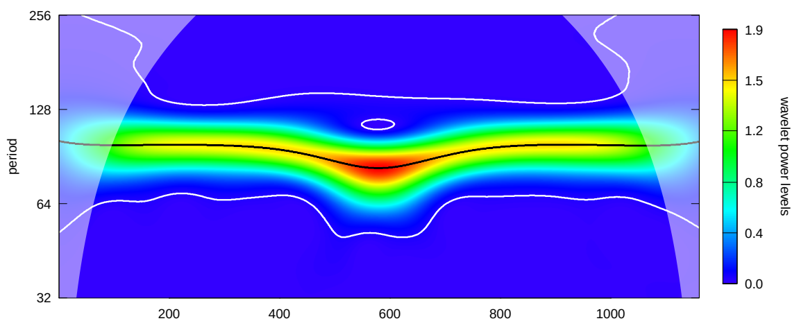
Figure 16: Power spectrum, method = "white.noise"
