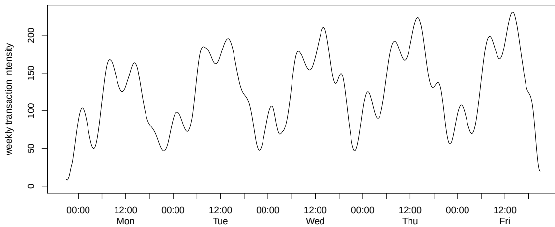
Figure 40: Transaction intensity estimate
