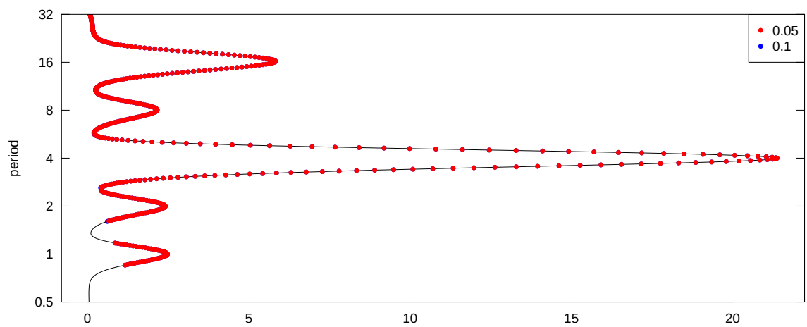
Figure 23: Cross-wavelet average power
