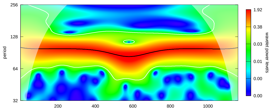
Figure 18: Power spectrum, color.key = "quantile"
