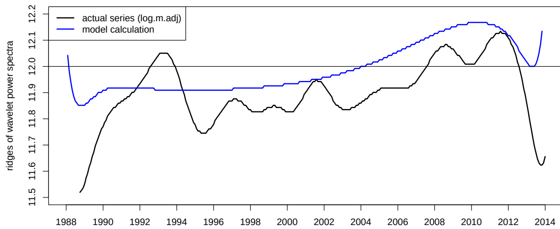
Figure 45: Ridge of power spectra
