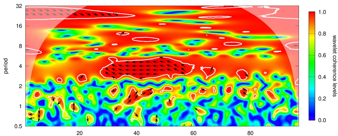
Figure 33: Wavelet coherence, window type: Bartlett
