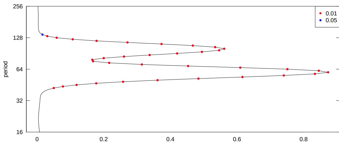
Figure 14: Average power, series y
