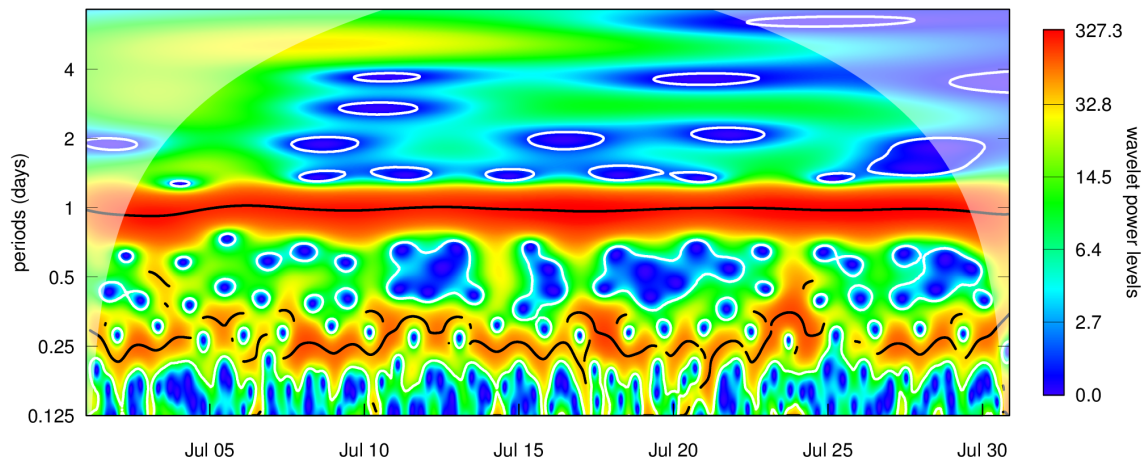
Figure 38: Transactions (active time only), the wavelet power spectrum
