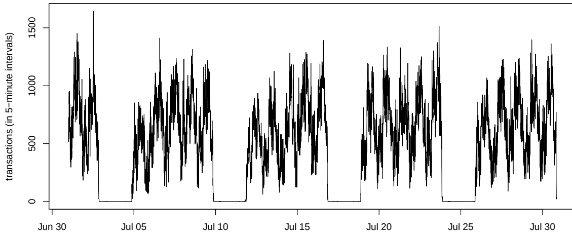
Figure 36: Number of transactions in five-minute intervals
