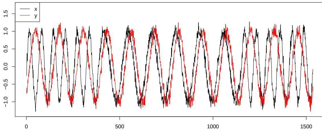
Figure 24: Series with joint period 128 at some time range, but different phase
