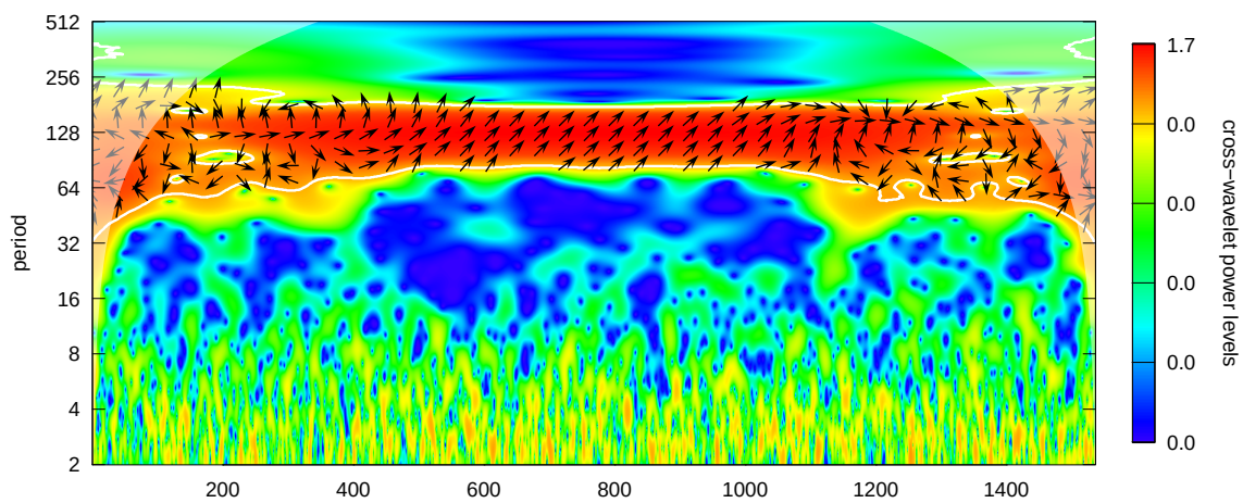
Figure 25: Cross-Wavelet power spectrum of the series
