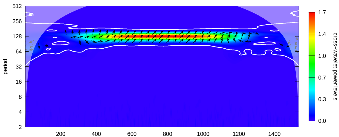
Figure 26: Cross-Wavelet power spectrum of the series with interval color key and restricted arrow area
