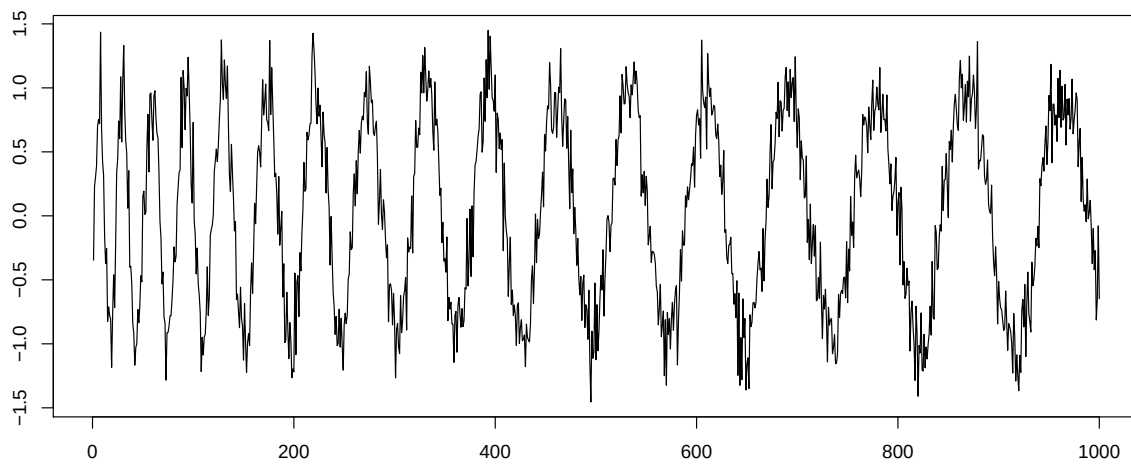
Figure 6: A series with nonconstant period
