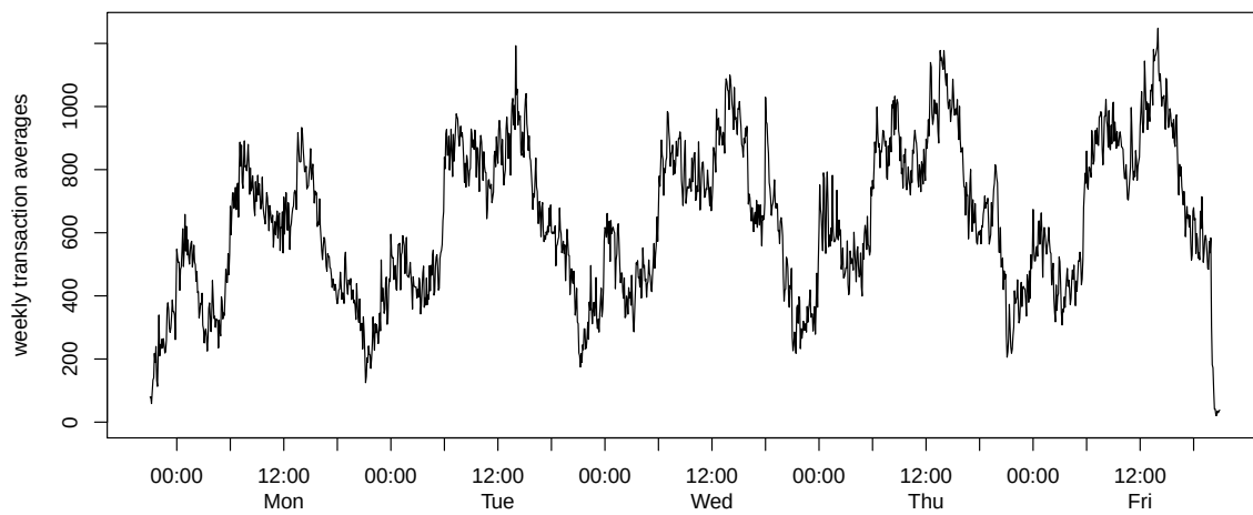
Figure 41: Transactions: weekly averages
