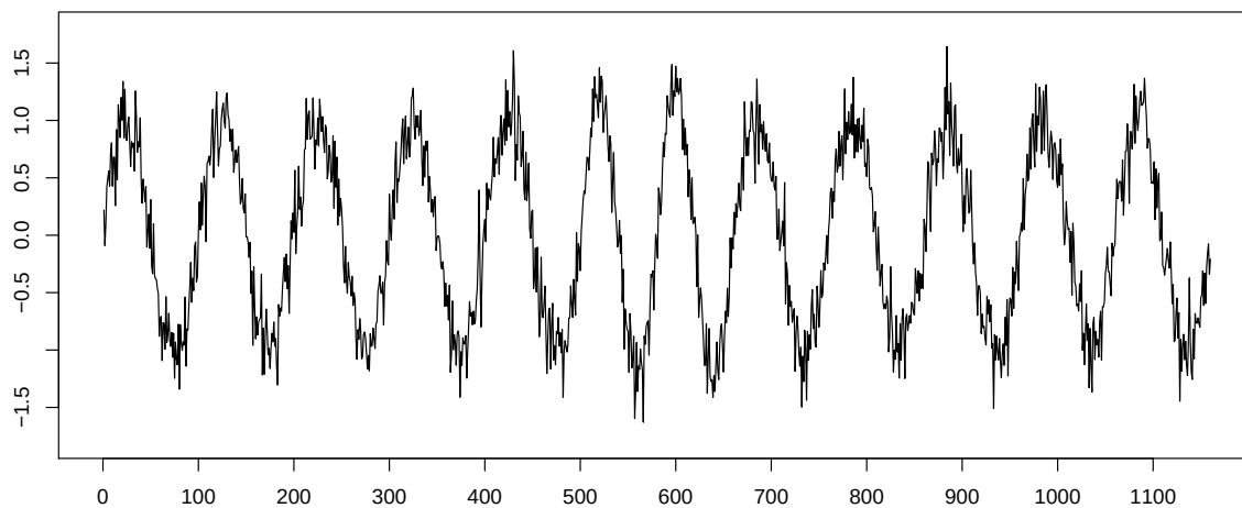
Figure 15: Time series with periods 80 (in the middle) and 100
