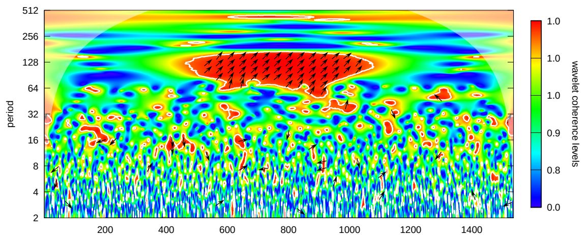
Figure 27: Wavelet coherence of the series
