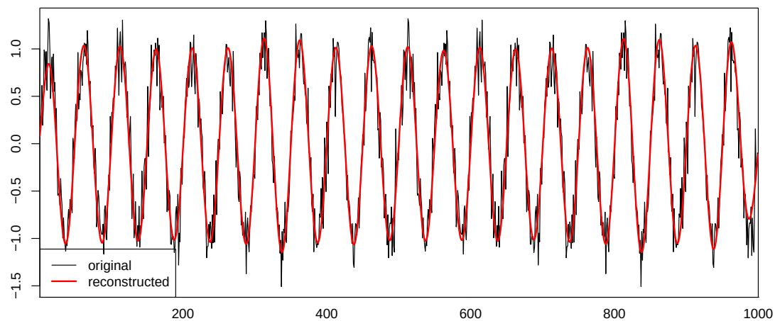
Figure 5: Reconstruction of the series
