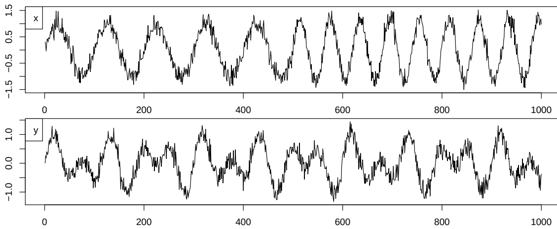
Figure 12: Two series with distinct periods
