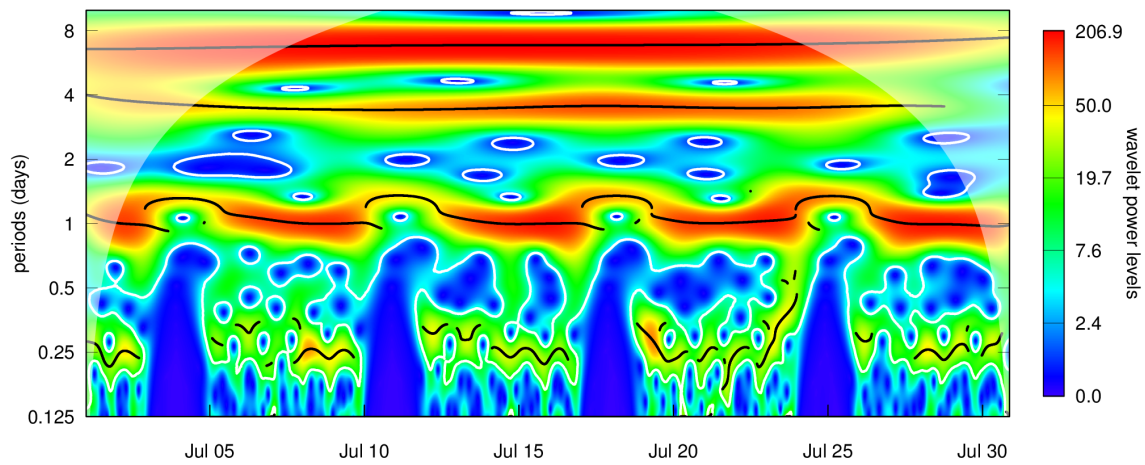
Figure 37: Transactions (original series), the wavelet power spectrum
