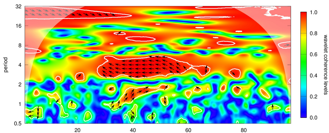
Figure 34: Wavelet coherence, window type: Boxcar
