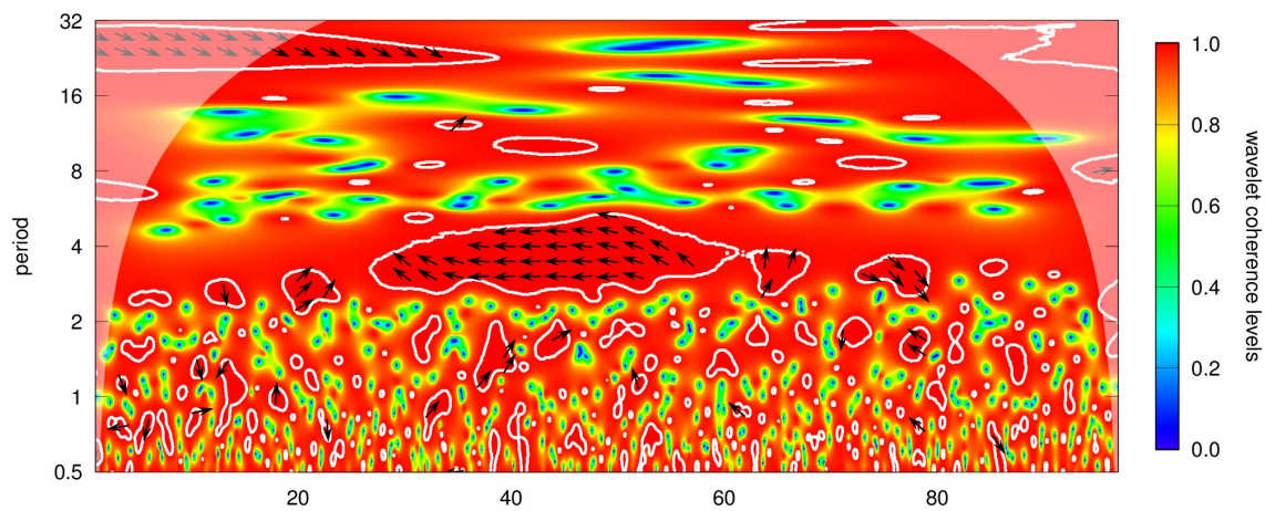
Figure 35: Wavelet coherence, no smoothing along time axis
