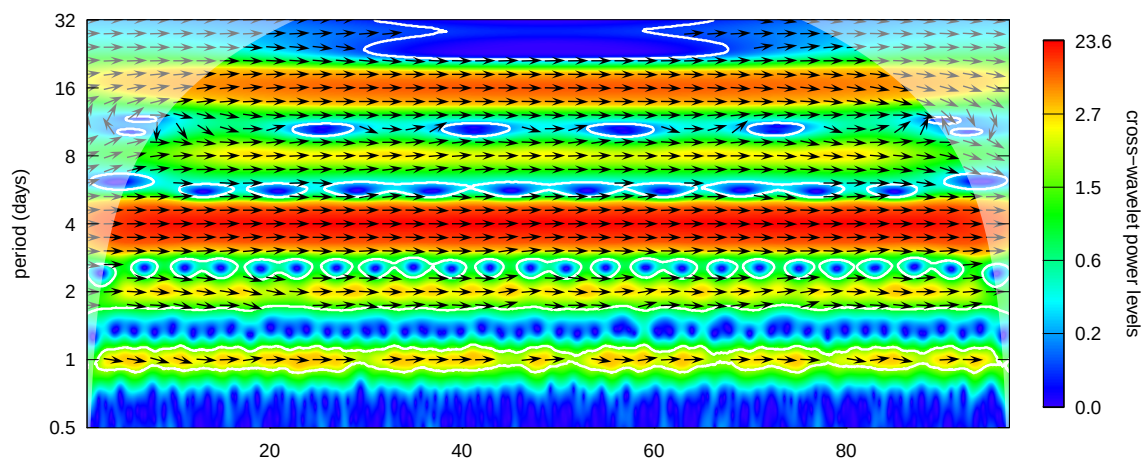
Figure 22: Cross-wavelet power spectrum of x and y
