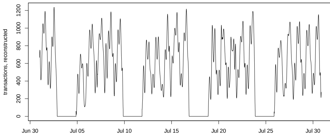
Figure 39: Number of transactions, reconstructed
