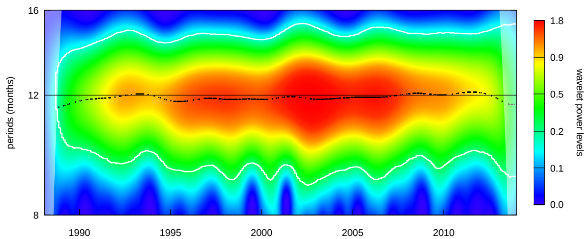
Figure 44: Marriages, the wavelet power spectrum, periods 8 – 16
