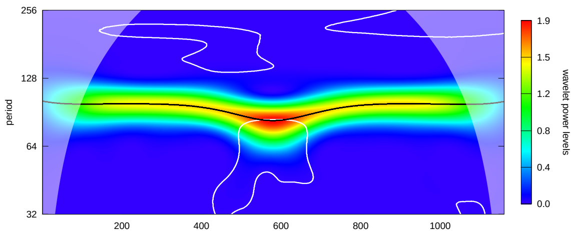
Figure 17: Power spectrum, method = "Fourier.rand"
