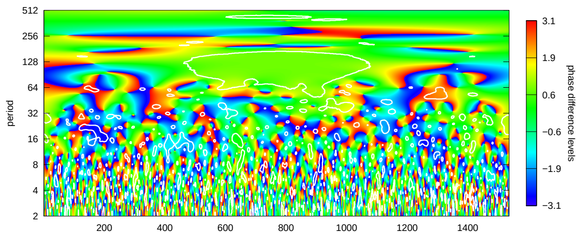
Figure 29: Phase difference image
